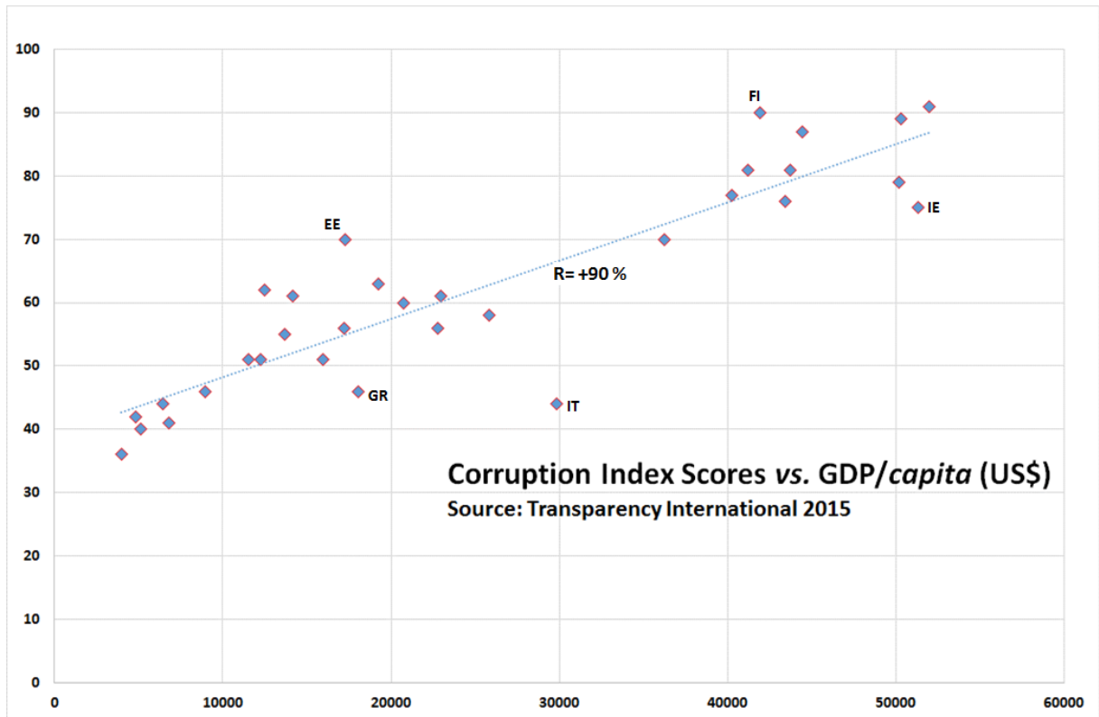
Figure 1.3.28b Corruption scores vs. GDP/capita. On the corruption scale, a score of 100 denotes a corruption-free country; the lower the score, the more severe the corruption. There is a quite close correlation ( R = 90\% ) between poverty and corruption. Deviating negatively ( i.e. more corrupt than should be expected) are Italy, Greece and Ireland. Very honest, in relation to their economic means, are Estonia and Finland. The three rich countries LUX, CH and NO have been left out – their GDP/capita is 50 – 100% higher than that of any other country.
